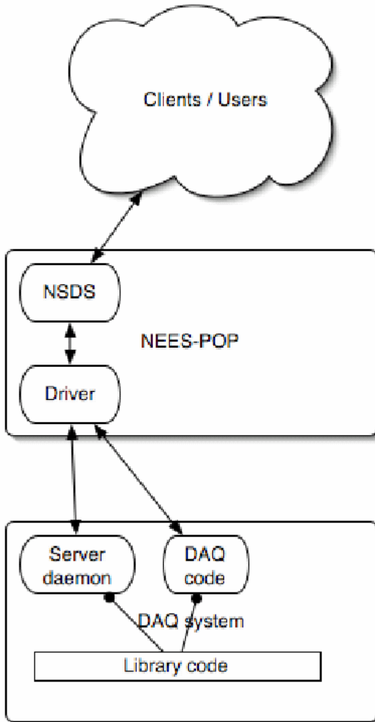
Figure 1: Interactions of NSDS, driver, and DAQ.
