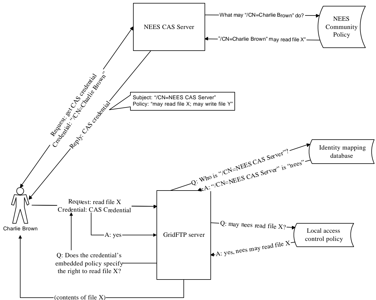
Figure 8: Using CAS with GridFTP
