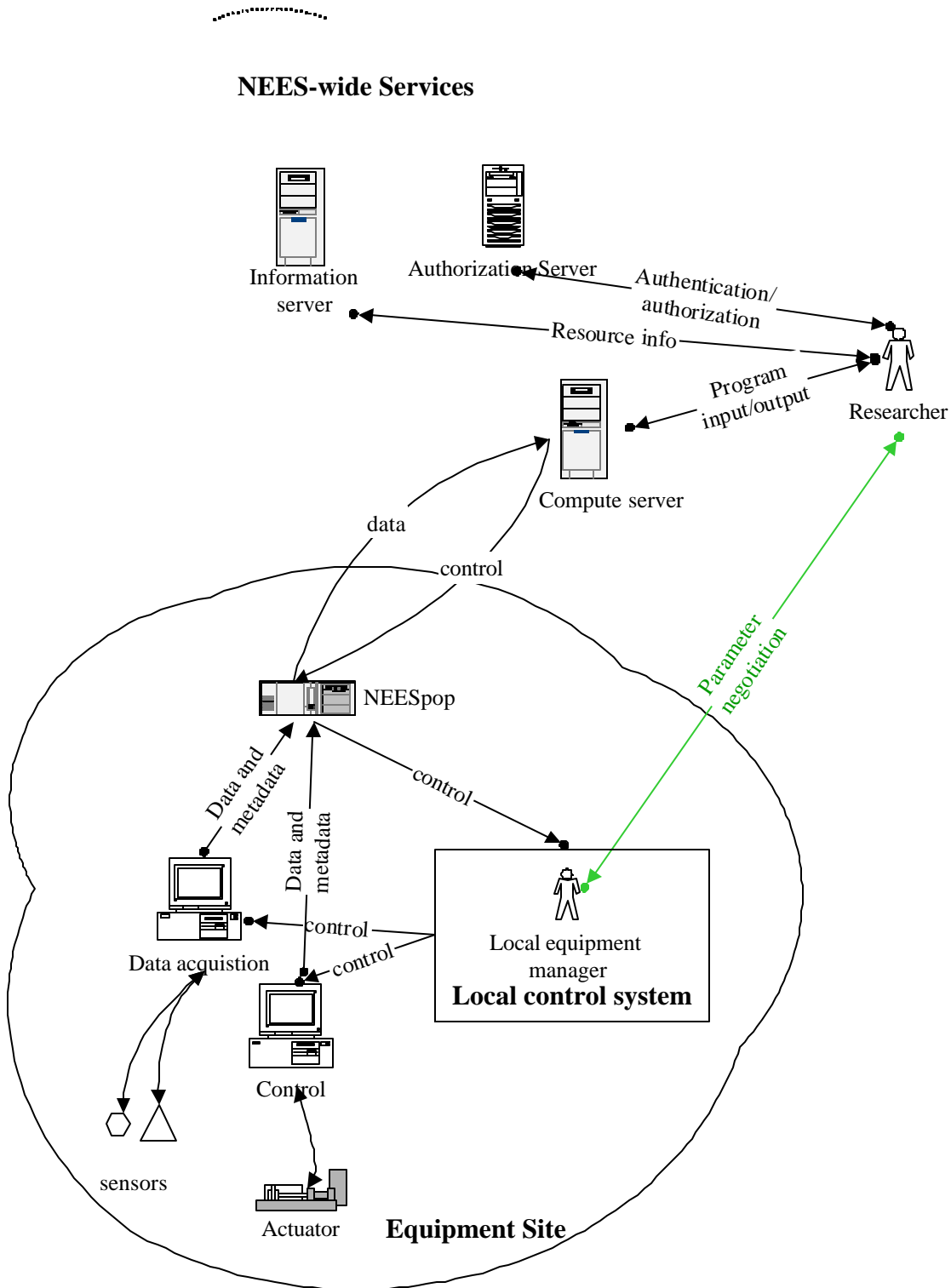
Figure 17: A pseudo-dynamic experiment
