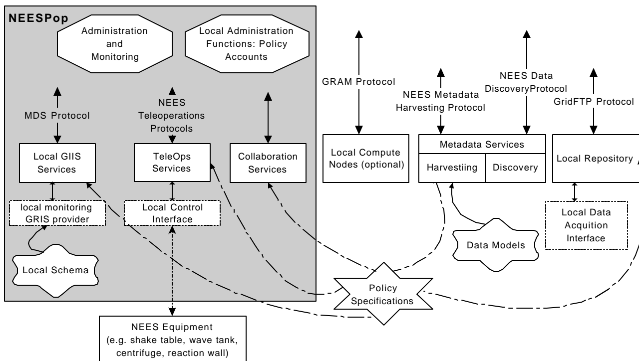
Figure 5: Details of NEESgrid architecture from the perspective of an equipment site.
