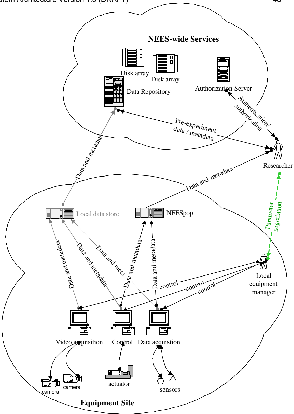
Figure 16: Monitoring an experiment trial in progress
