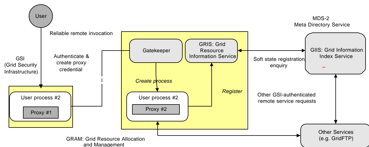
Figure 3: Overview of primary Globus services and protocols.
