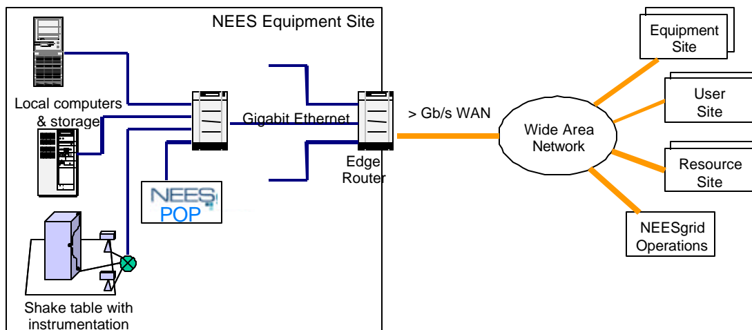
Figure 6: NEESgrid schematic, showing an equipment site on the left, with its NEES-POP, and wide area links to other NEES resource and user sites.
