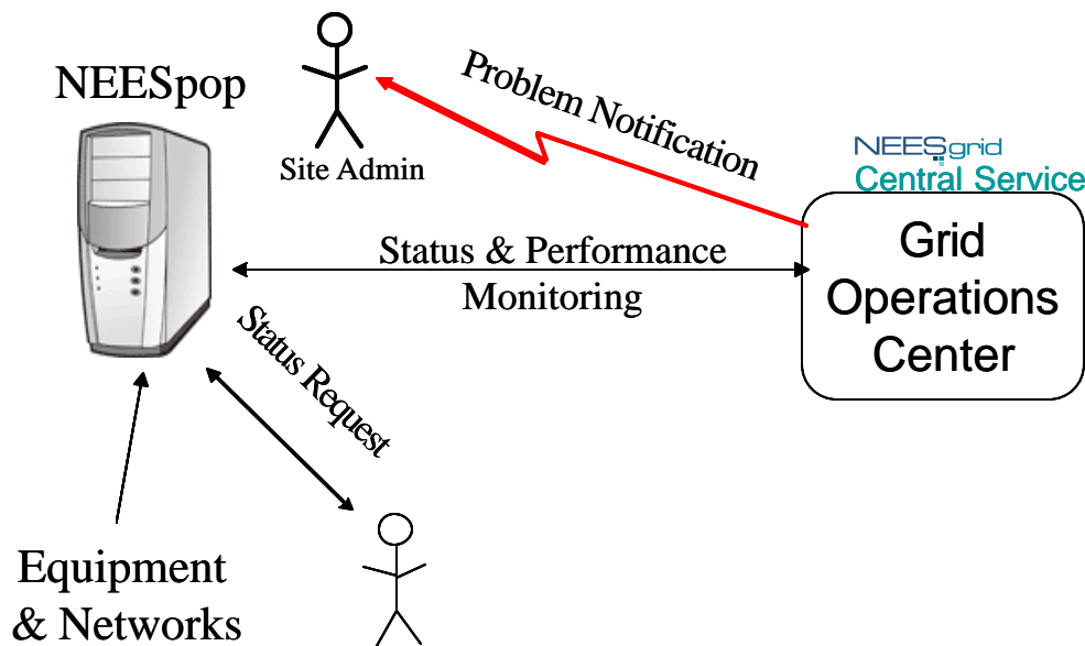
Figure 14: NEESgrid administrative structure for monitoring NEES sites
