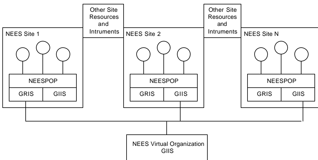
Figure 9: NEESgrid resource discovery architecture
