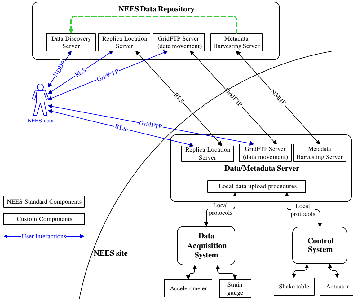
Figure 10: Data acquisition and conversion in NEESgrid
