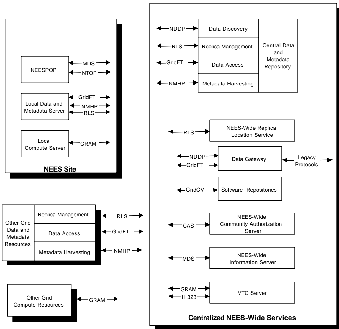
Figure 4: Global structure of the NEESgrid system architecture.
